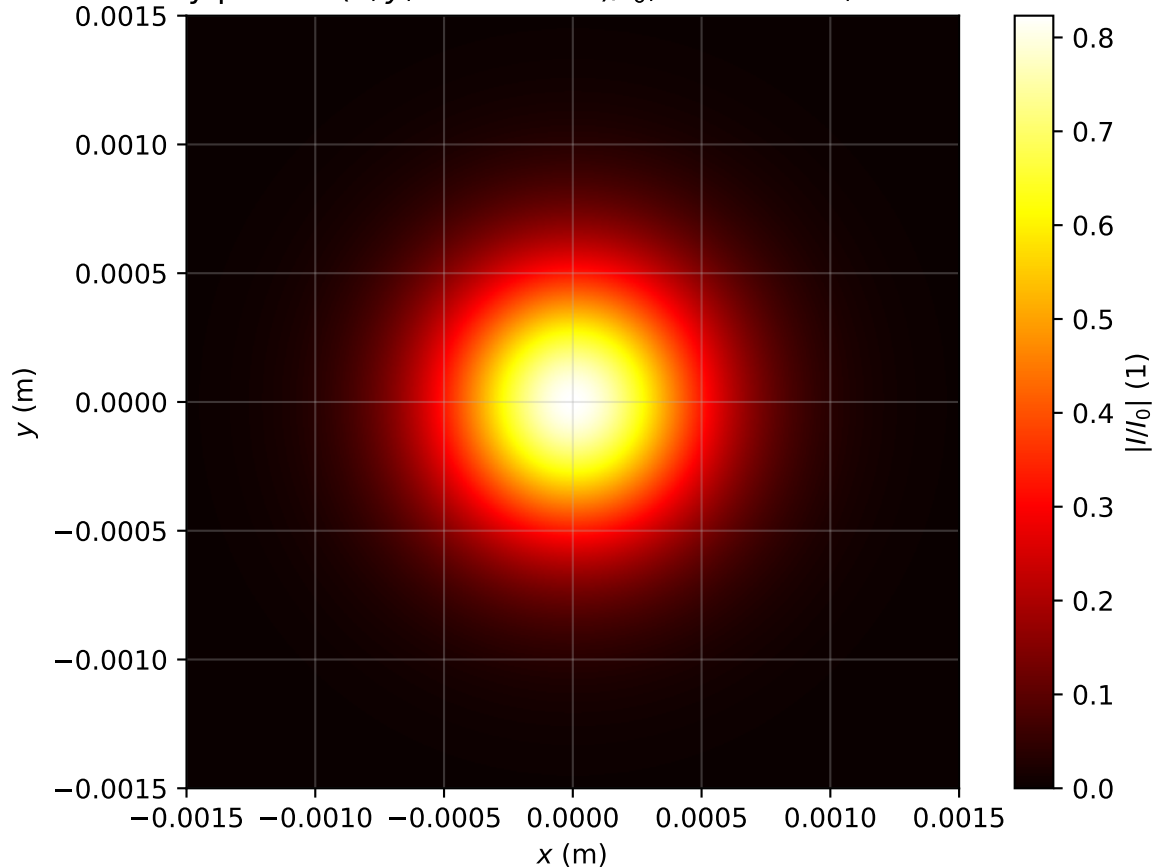
Intensity profile I(x, y, z = 1.672m)/I_0 , \text{Pin}=0.4\text{Pcr} , artificial time
